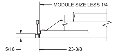
PV-NR, CURVED BLADE, PERFORATED FACE, 24" x 24" LAY-IN PANEL, NARROW REGRESS
